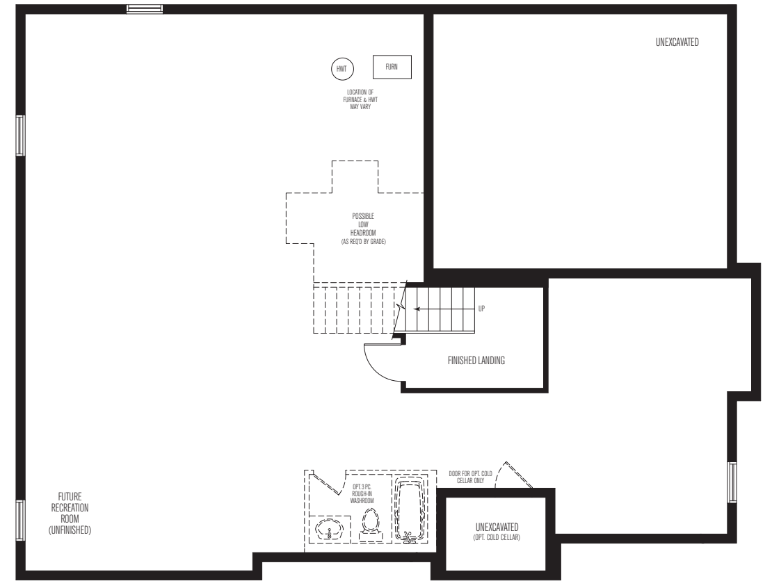
BASEMENT FLOOR ELEV. B
