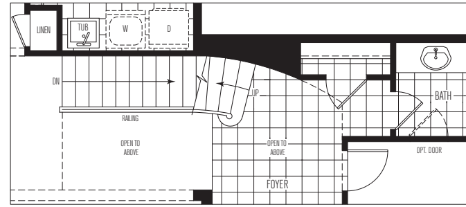
PART GROUND FLOOR FOR OPT. LOFT ELEV. A
