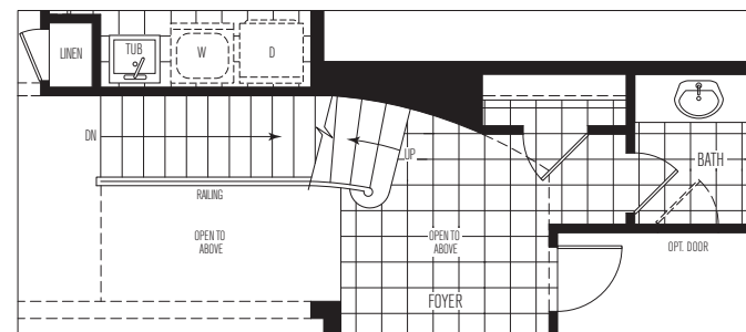
PART GROUND FLOOR FOR OPT. LOFT ELEV. B
