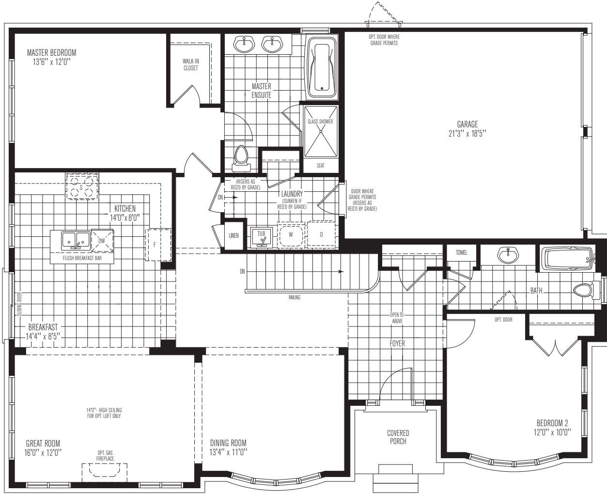
GROUND FLOOR ELEV. A
