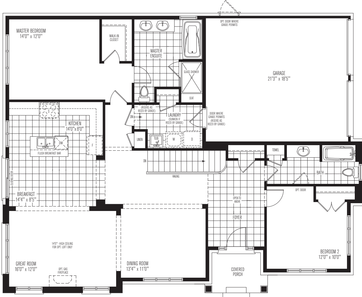
GROUND FLOOR ELEV. B
