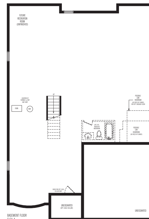
BASMENT FLOOR ELEV. A
