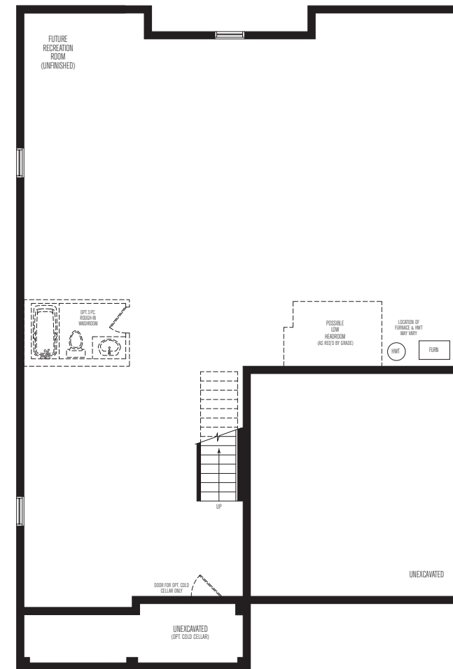
BASEMENT FLOOR ELEV. A
