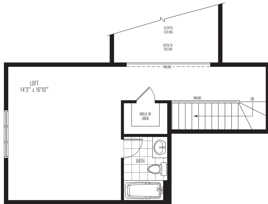
OPT. LOFT PLAN
